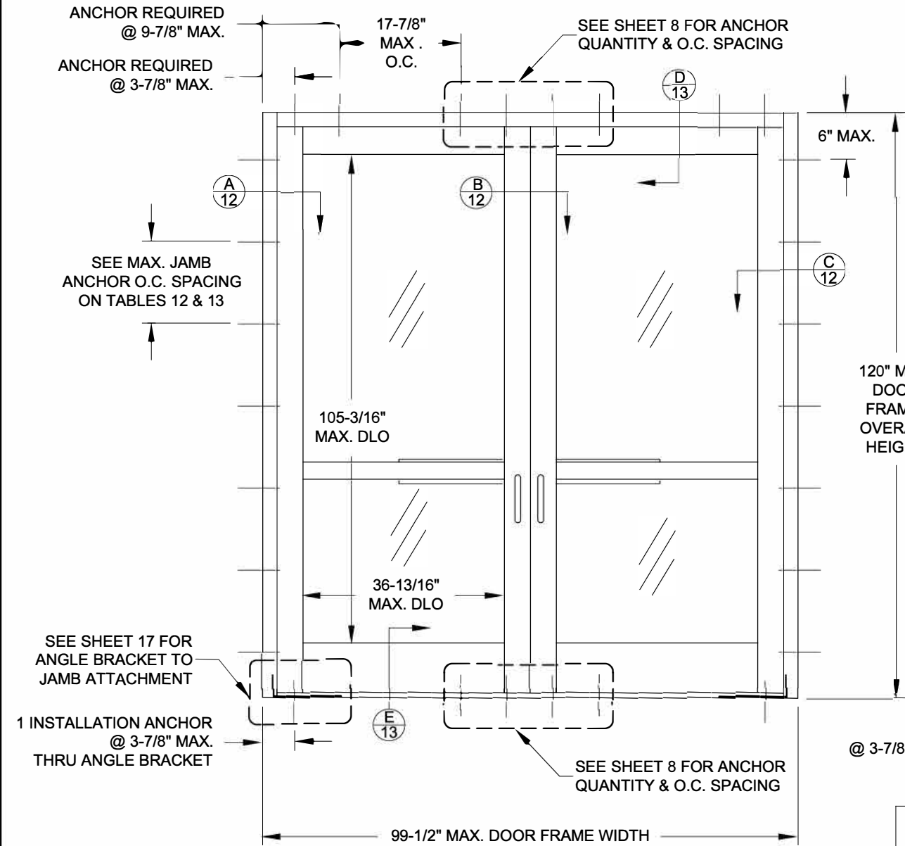
TYP. ELEVATION OF DOUBLE DOOR WITHOUT TRANSOM
