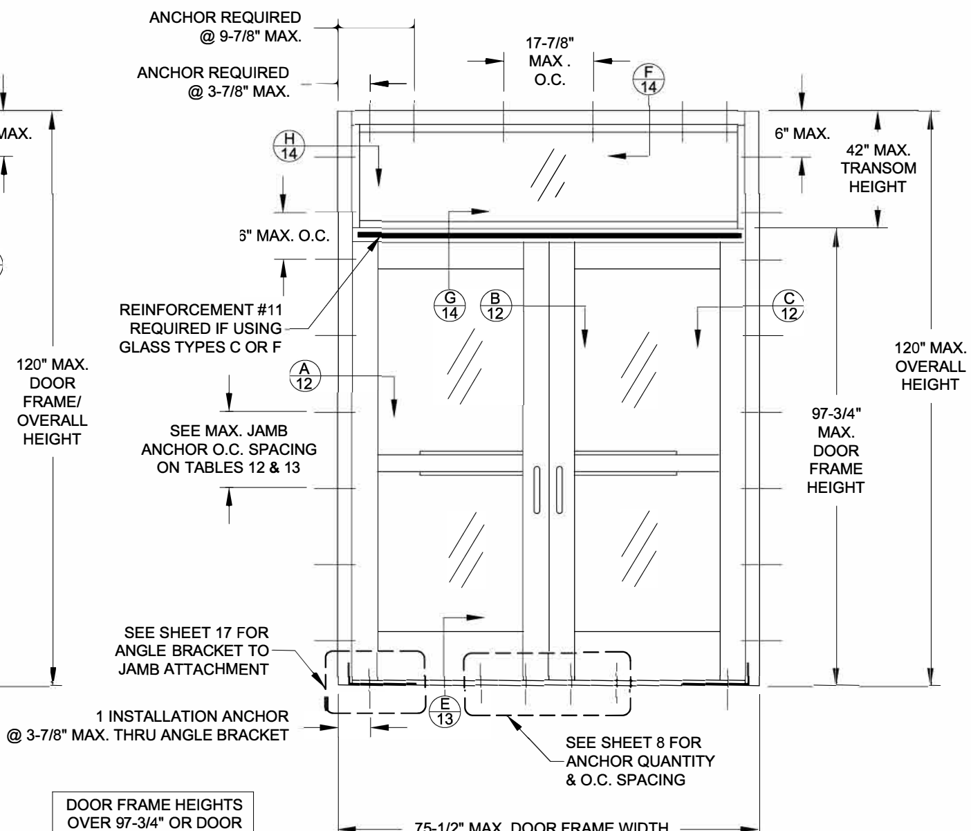
TYP. ELEVATION OF DOUBLE DOOR WITH TRANSOM
