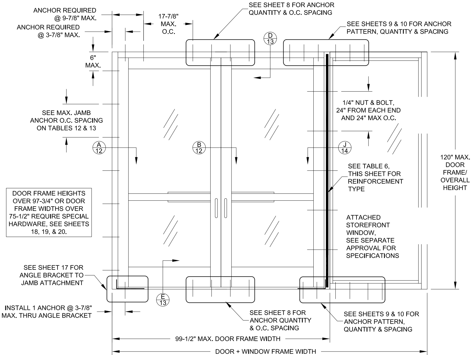
TYP. ELEVATION OF DOUBLE DOOR WITHOUT TRANSOM, ATTACHED TO STOREFRONT WINDOW
