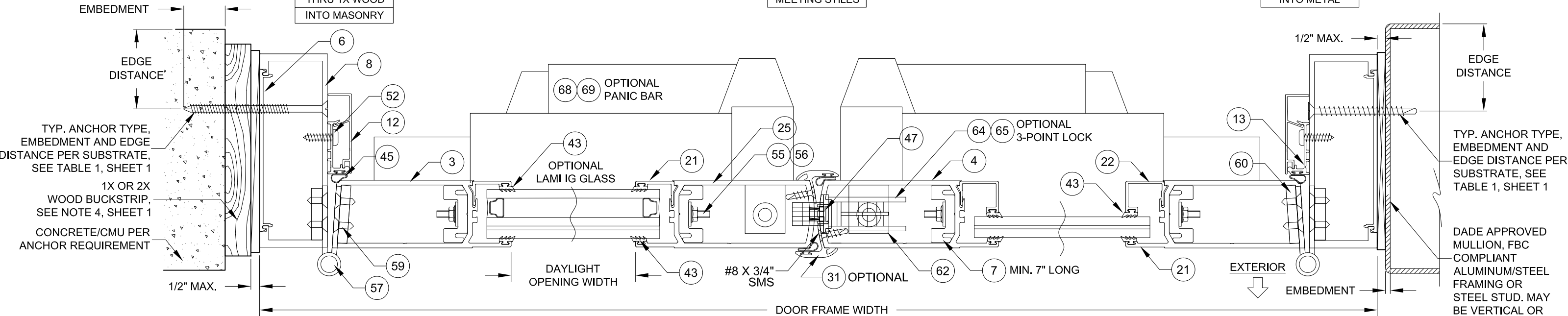
HORIZONTAL SECTION (DOUBLE DOOR)
