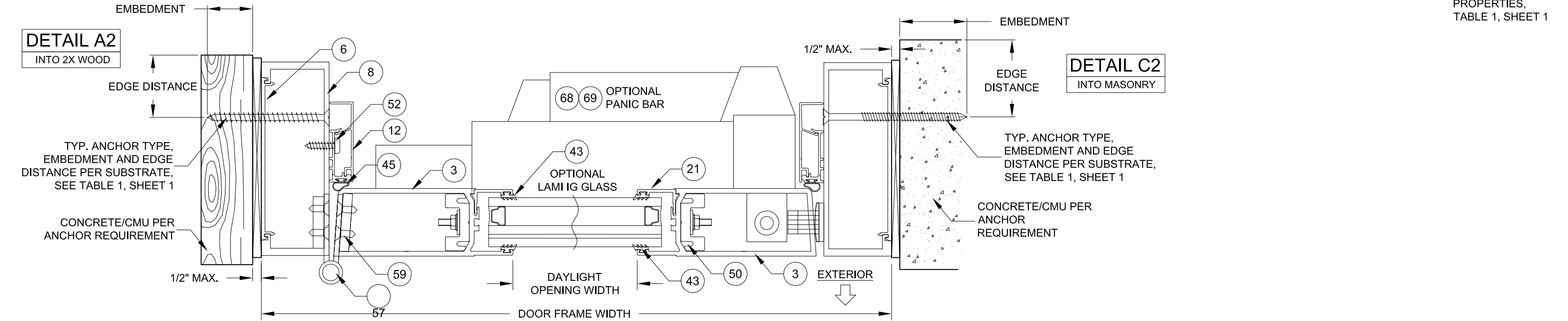
HORIZONTAL SECTION (SINGLE DOOR)
