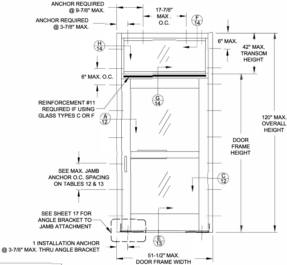
TYP. ELEVATION OF SINGLE DOOR WITH TRANSOM
